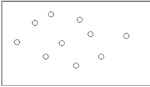
Figure 3.78: A scatterplot.
