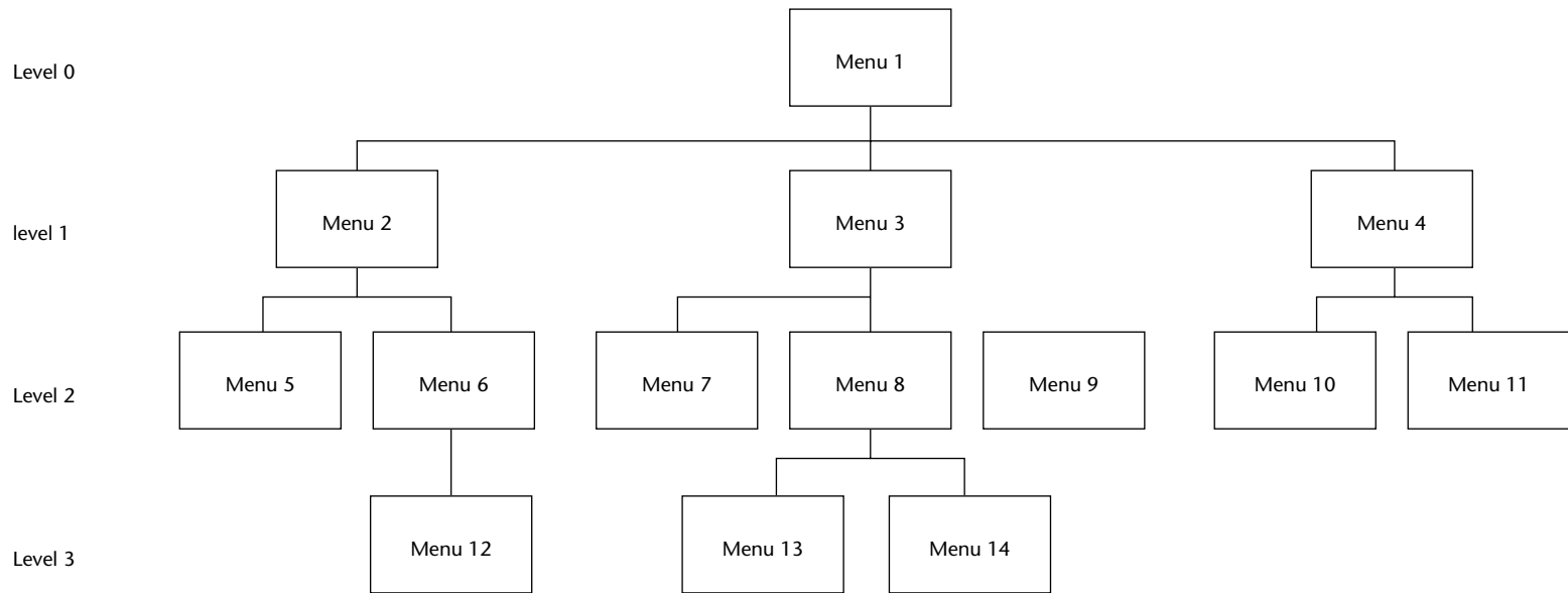
Figure 4.4: Hierarchical or sequential menus.
