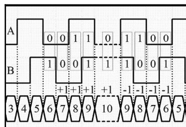
Detecting motor direction from encoder pulses
