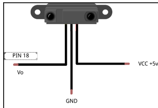
Pinout of Sharp IR sensor
