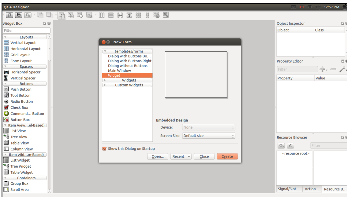
Qt 4 Designer
