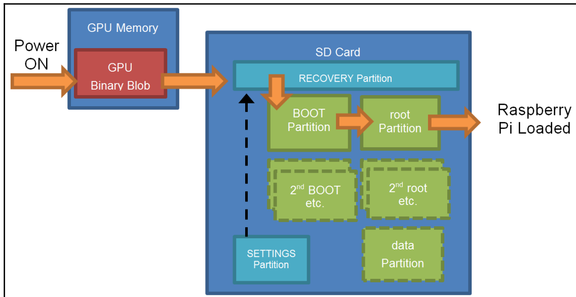
NOOBS creates several partitions on the SD card to allow the installation of multiple operating systems and to provide recovery
