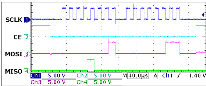
The SPI signals: SCLK (1), CE(2), MOSI(3), and MISO(4)
