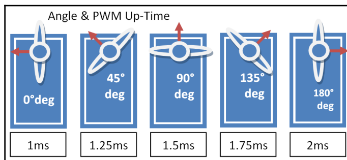
The servo angle is controlled by sending a PWM Up Time between 1 ms and 2 ms
