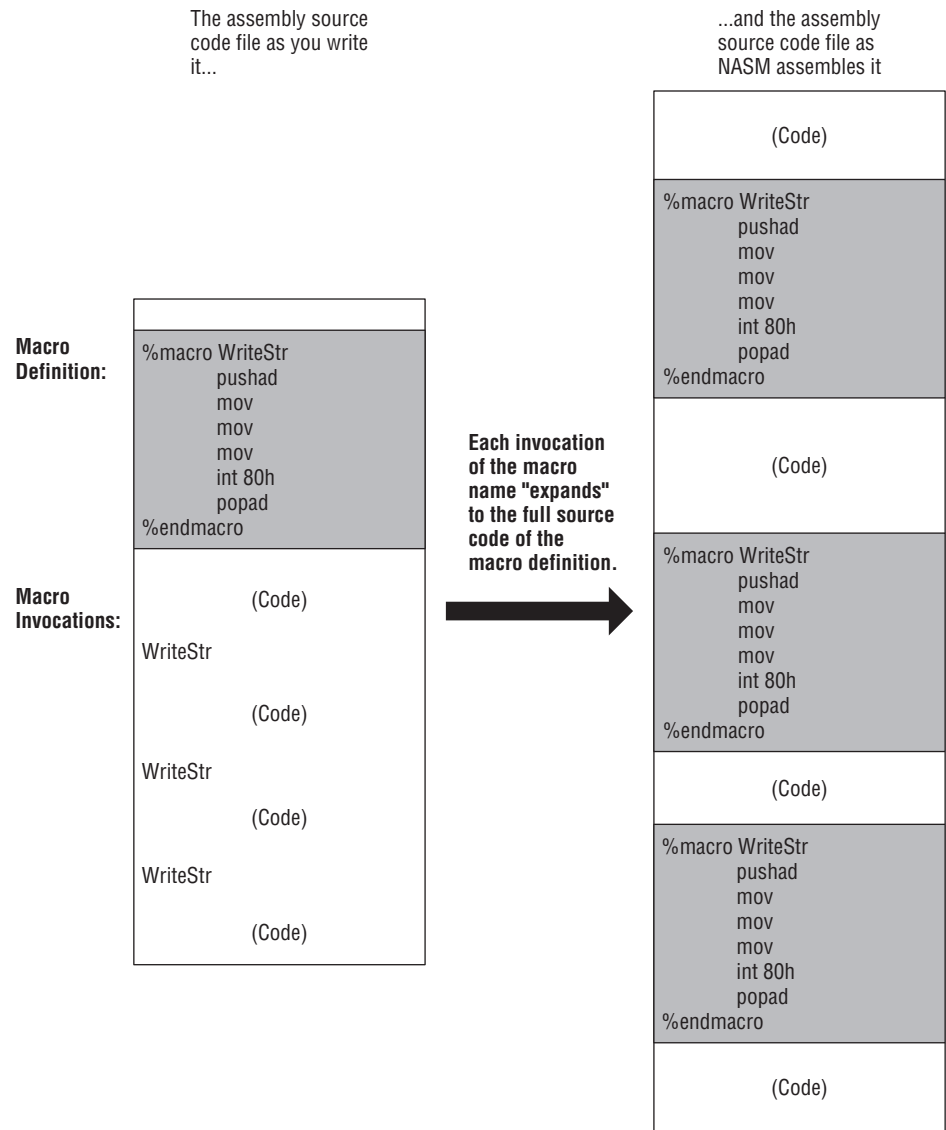
Figure 10-4: How macros work
