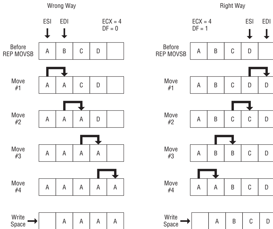
Figure 11-2: Using MOVSB on overlapping memory blocks
