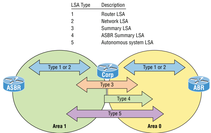
FIGURE 19.5 Basic LSA types
