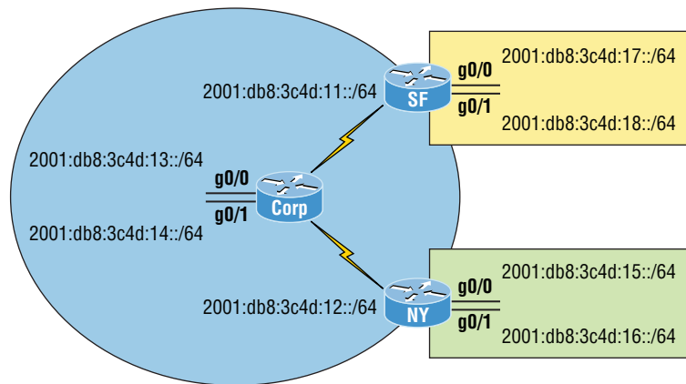
FIGURE 19.11 Configuring OSPFv3
