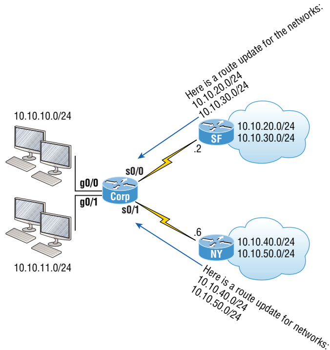
FIGURE 17.8 Split horizon in action, part 1
