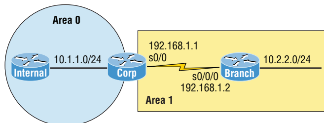
FIGURE 19.9 Our internetwork
