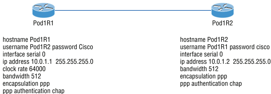
FIGURE 21.15 Failed PPP authentication
