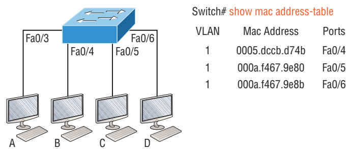
FIGURE 10.3 Forward/filter table
