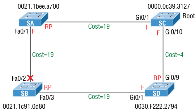
FIGURE 15.12 RSTP example 1 answer
