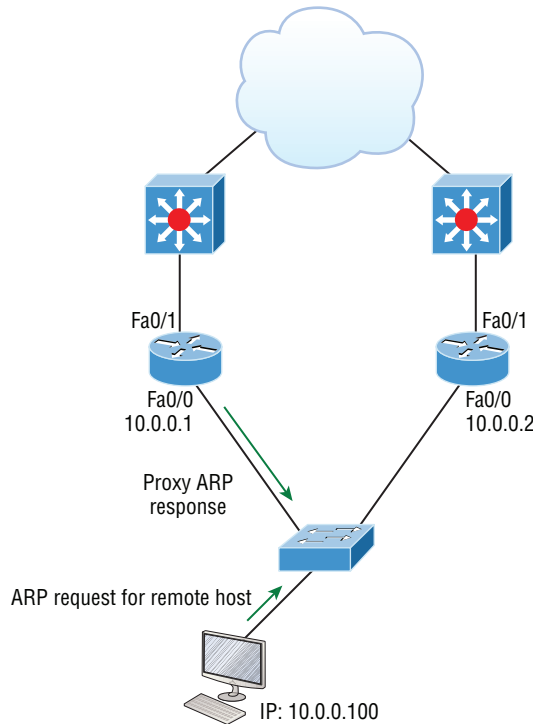
FIGURE 16.7 Proxy ARP
