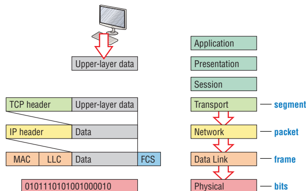
FIGURE 2.21 Data encapsulation
