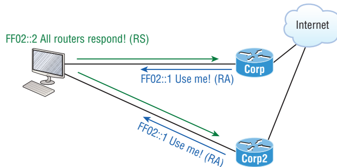
FIGURE 20.5 Router solicitation (RS) and router advertisement (RA)
