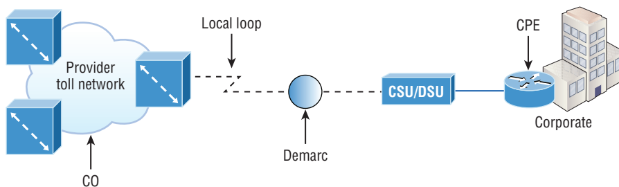
FIGURE 21.4 WAN terms
