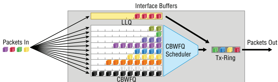
FIGURE 22.16 Queuing mechanisms
