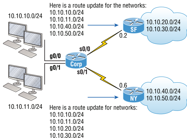
FIGURE 17.9 Split horizon in action, part 2
