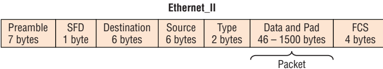
FIGURE 2.8 Typical Ethernet frame format
