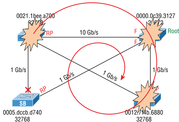
FIGURE 15.18 STP failure
