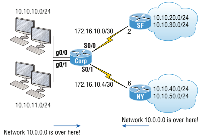
FIGURE 17.6 Discontiguous networks
