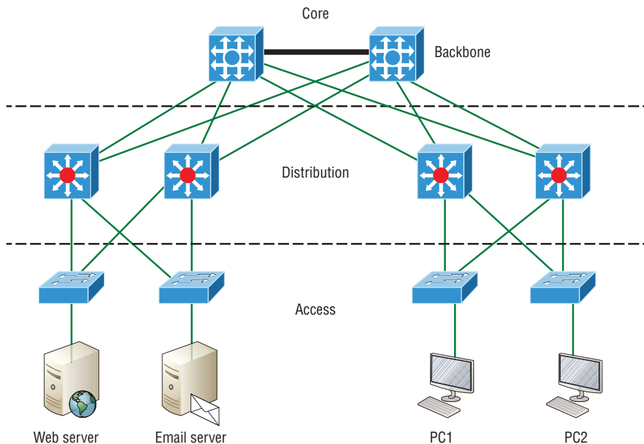
FIGURE 2.24 The Cisco hierarchical model
