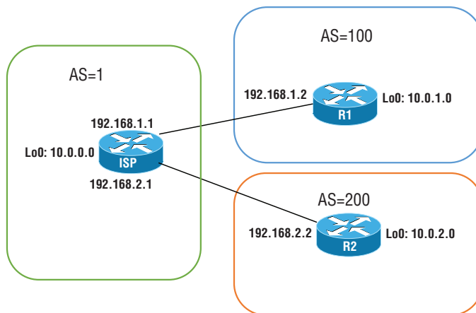
FIGURE 21.25 Example of EBG lay layout
