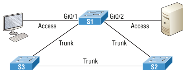
FIGURE 15.19 PortFast
