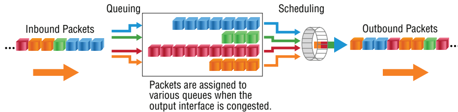
FIGURE 22.15 Congestion management
