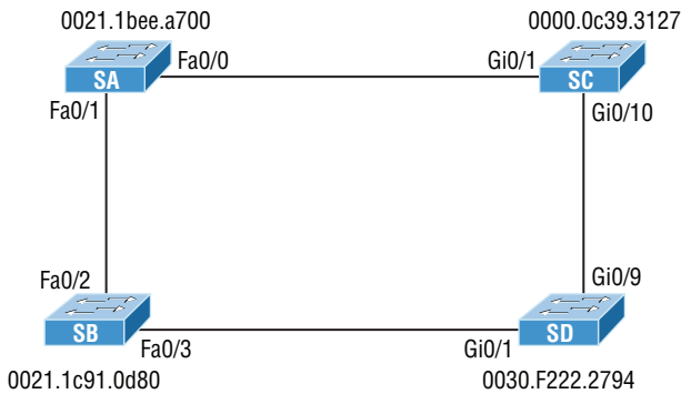
FIGURE 15.11 RSTP example 1
