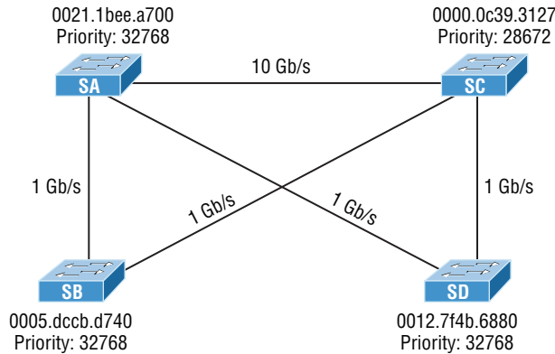
FIGURE 15.13 RSTP example 2
