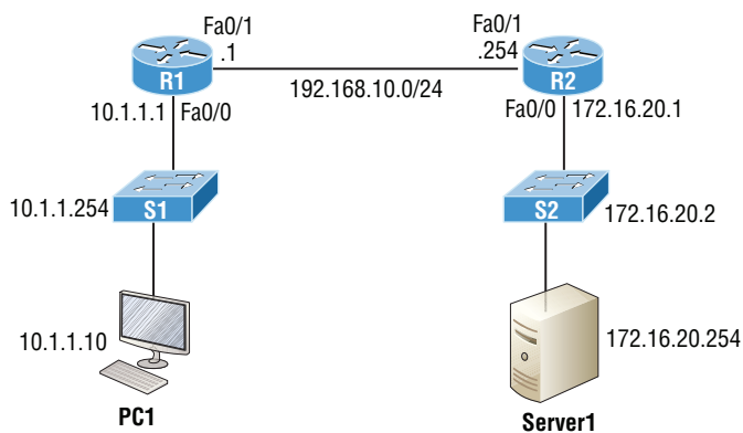
FIGURE 20.1 Troubleshooting scenario
