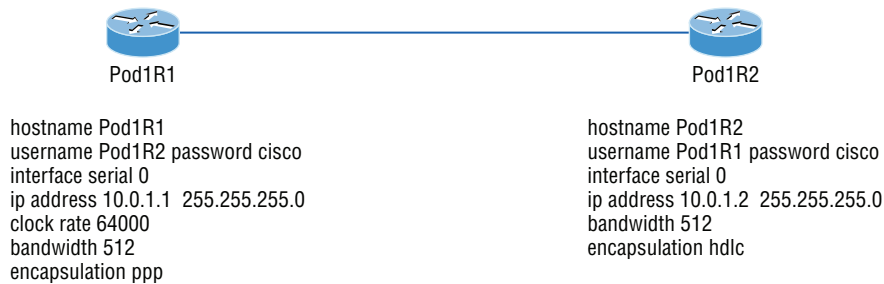
FIGURE 21.16 Mismatched WAN encapsulations
